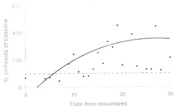
Figure 2. Example of a trendline (solid line) for postmovement corticoid concentrations in a cheetah. The dashed line at 100% represents the baseline (premovement average). All values are represented as a percentage of baseline. This animal's corticoid concentration remained above baseline for at least 30 days.
